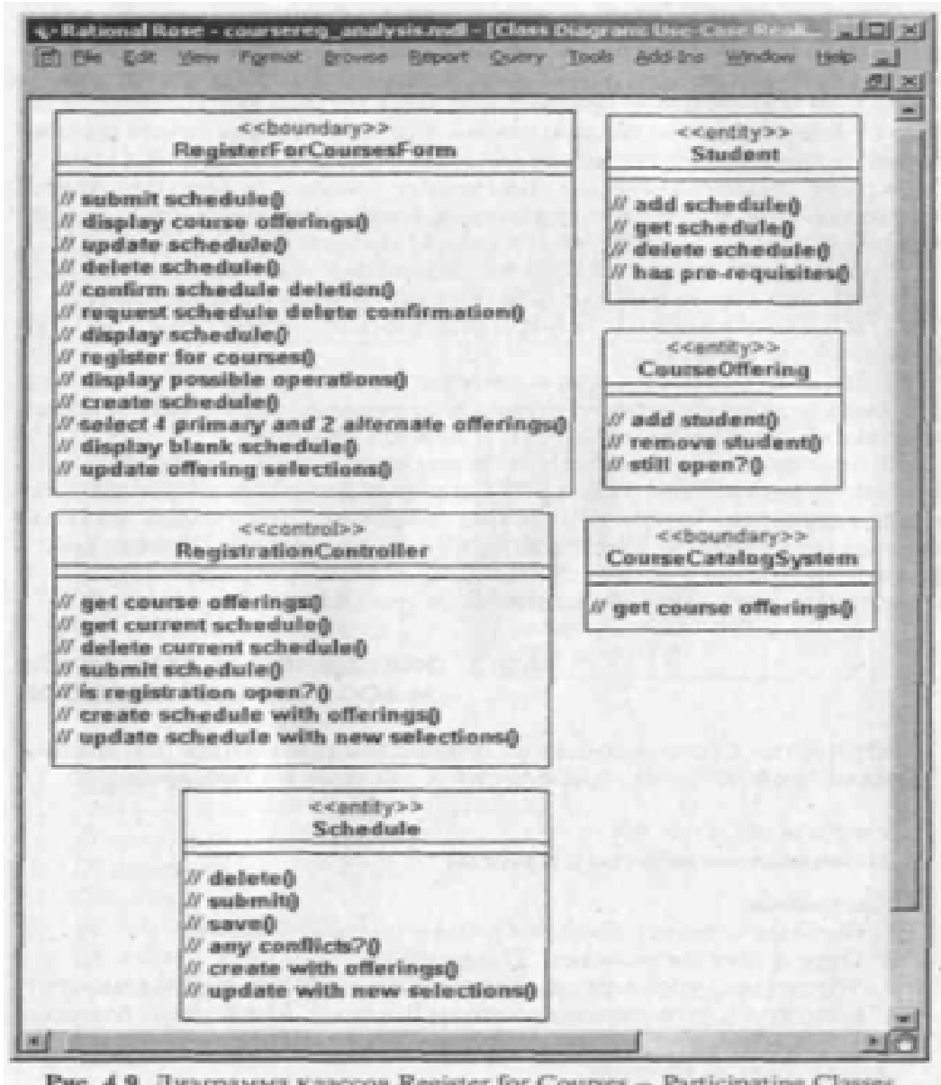
FIG. 4.9. UML CLASS DIAGRAM: Register for Courses – Participating Classes
